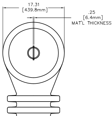
PAD CONFIGURATION FOR 800:5-1200:5 1 PAD EACH SIDE
