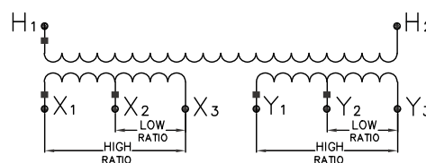
Dual-Tapped Secondary (Six secondary terminals)
