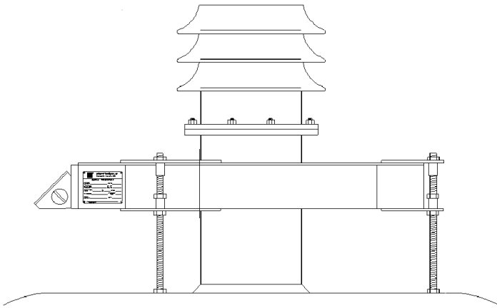
Figure 1. Slip-over cast resin BCT installed over outdoor bushing Note - BCT to be installed below ground plane
