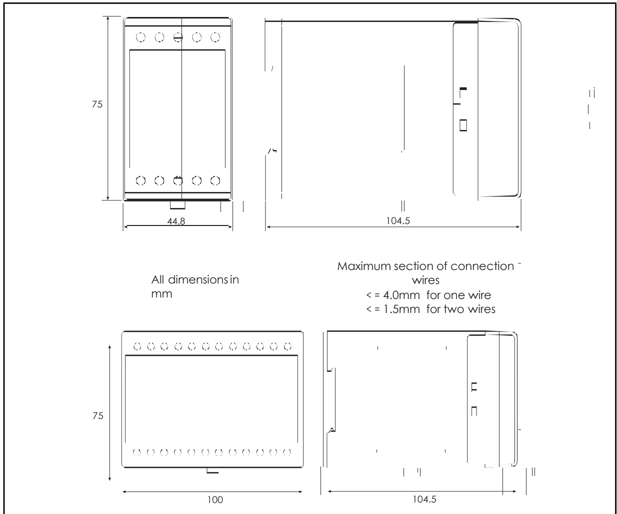
FIGURE 1 : I400 DIMENSIONS
