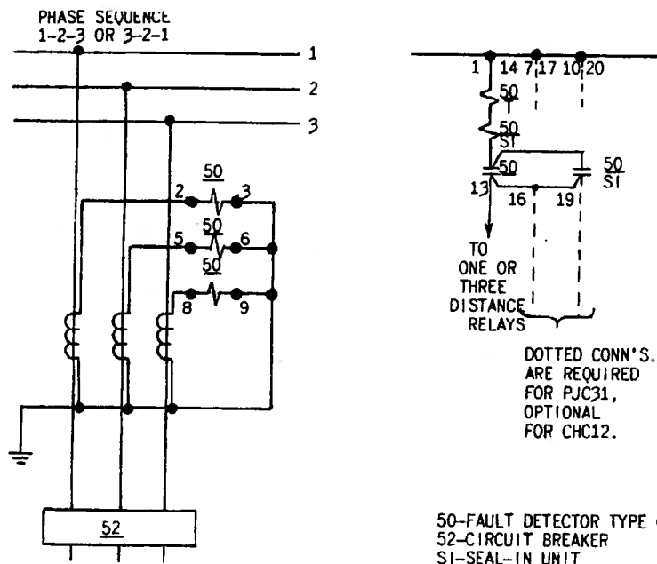
Fig. 2 (0165A6007-0) Typical External Connections For The CHC12A Relay
