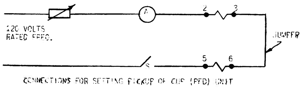
Fig. 6 (0165A6011- ) Test Connections For The PFD Unit Of The CHC12A Relay
