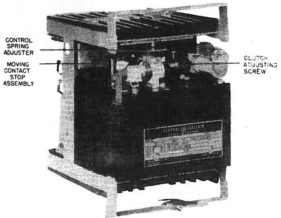
Fig. 1 (8030330 & 8030329) CHC12A Removed From Case
