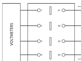
Voltage Test Block with Spring Loaded Contacts
