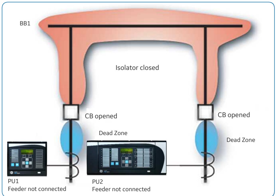
Fig. 7: Dead zone protection
