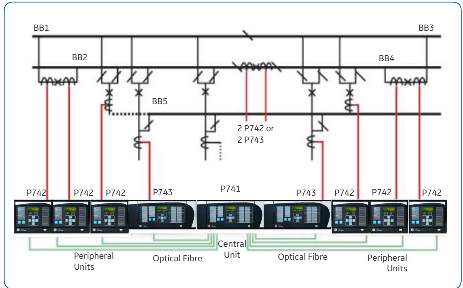
Fig. 1: P740 scheme applied to protecting a double busbar with transfer bus
