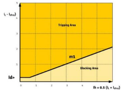
Figure 6 Defrost characteristics
