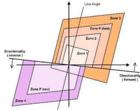
Figure 3: Quadrilateral characteristics
