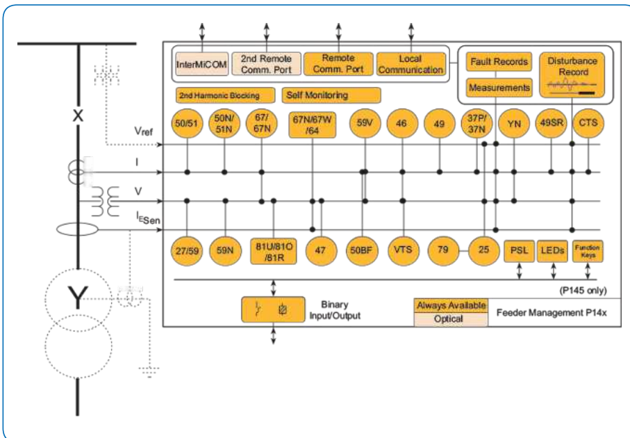
Functional overview ( See Protection Functions Overview for description of ANSI codes)
