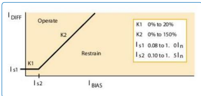
REF biased differential characteristics
