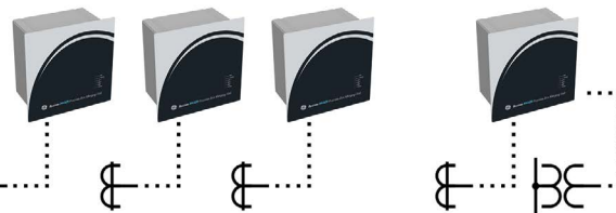
Process Bus: IEC61850-9-2LE or 61869* SV IEEE 1588 Grand Master or slave 61850-9-1 GOOSE
