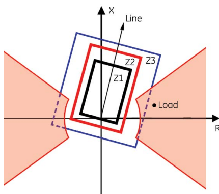
Distance relay quadrilateral characteristics supervised by the load encroachment function.
