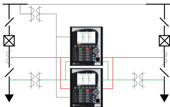
Redundant feeder
