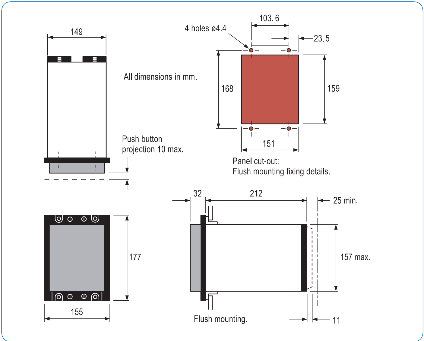
Figure 8 Case outline size 6
