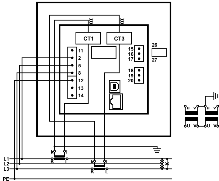
Connection 3u (2W3u)
