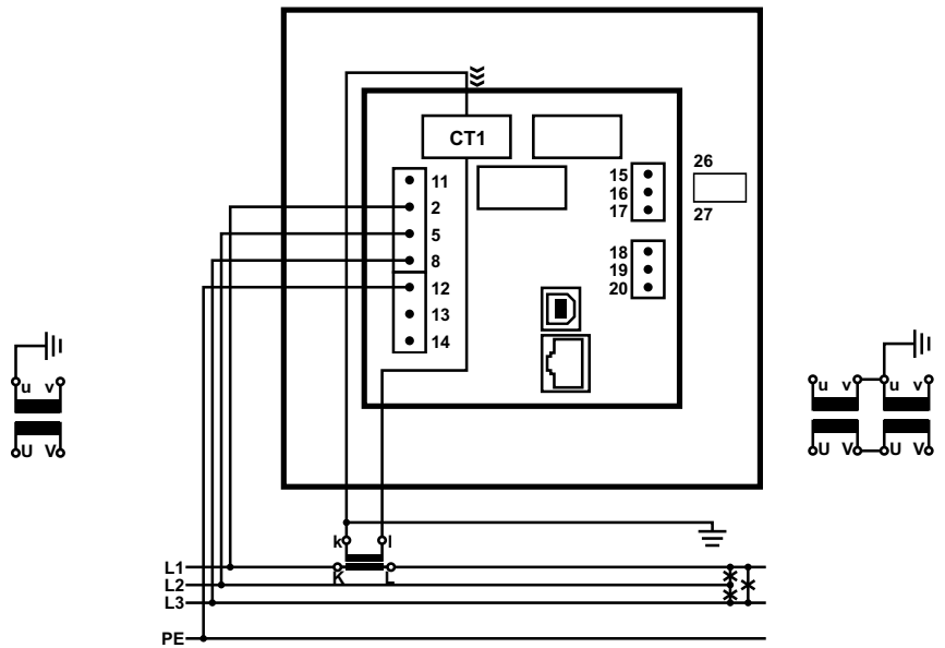
Connection 3b (1W3b) Three phase, three wire connection with balanced load
