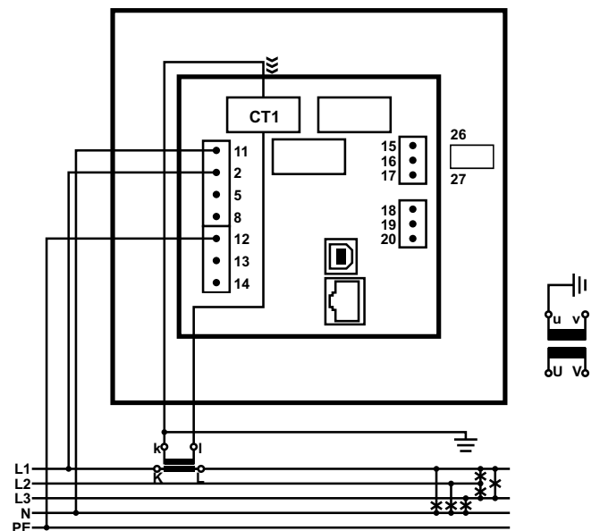
Connection 4b (1W4b)
