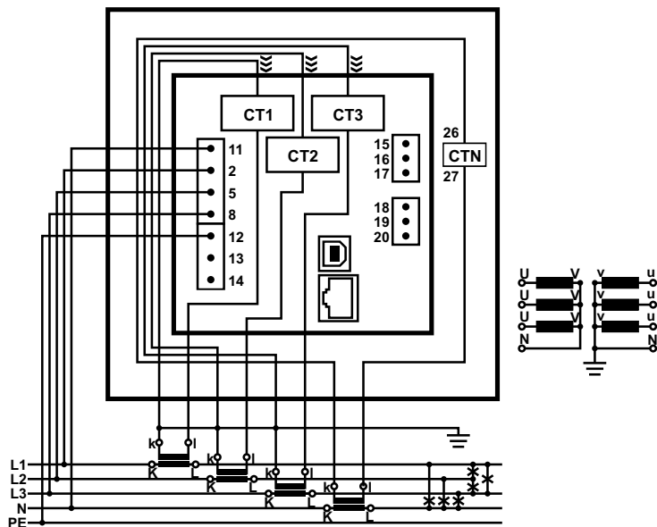
Connection 4u (3W4u)
