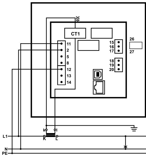
Connection 1b (1W) Single phase connection
