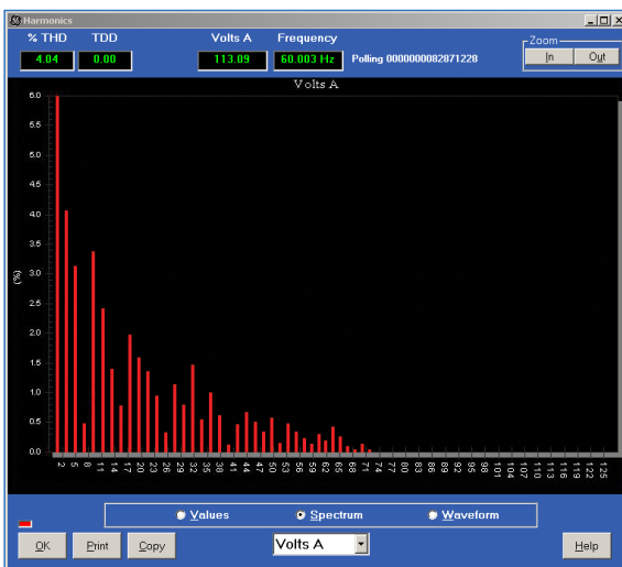
Harmonic Spectrum
