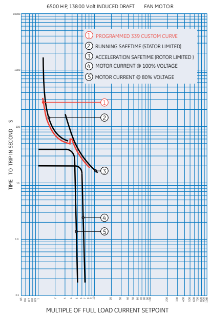
Typical Flexcurve
