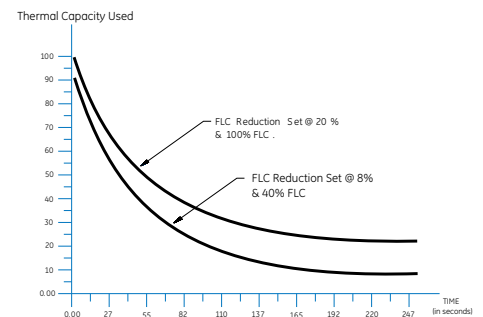
Motor cooling curves
