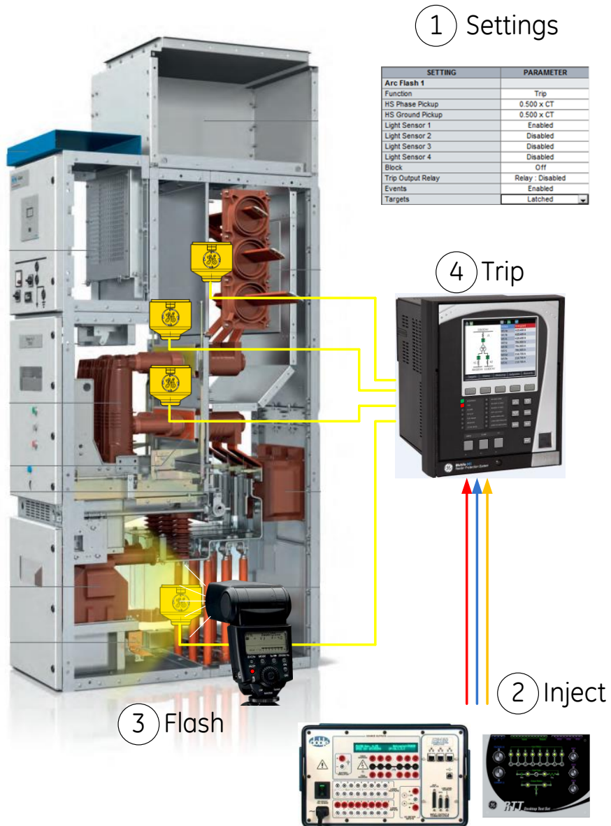
Figure 6. Arc Flash Testing with Secondary Injection
