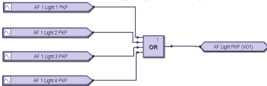
Figure 7. FlexLogic for Arc Flash Light Test
