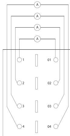
Current Test Plug SMTB4TPNLCN (Not wired) SMTB4TPWLCN (Pre-wired)
