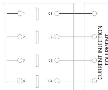
Current Test Plug SMTB4TPNLCW (Not wired) SMTB4TPWLCW (Pre-wired) (Plug shown with terminals 1, 2, 3, & 4 internally shorted)
