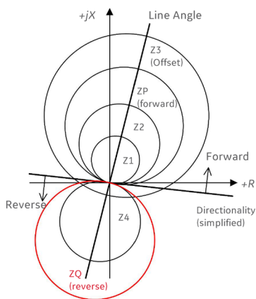
Figure 6: Mho characteristics
