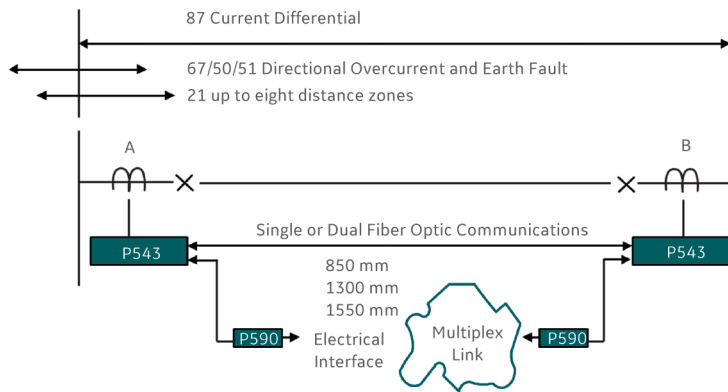
Figure 3a Application to 2 terminal lines
