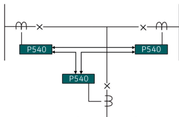
Figure 3b Upgrade to 3 terminal lines
