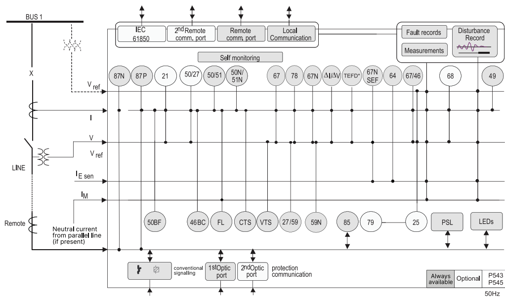
Figure 1: System overview of the P543 and P545 Firmware 92
