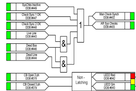
Figure 9 Programmable scheme logic
