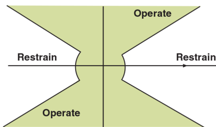
Figure 8 Load blinder
