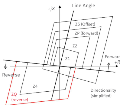
Figure 7: Quadrilateral characteristics
