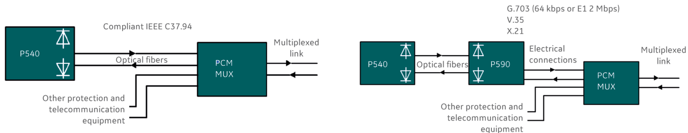
Figure 3d Multiplexed link - relay connected to a remote PCM multiplexer using optical fiber (IEEE C37.94™ compliant MUX) and via a P590 interface unit
