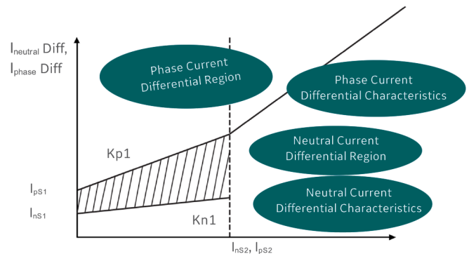
Figure 2: Differential protection characteristic
