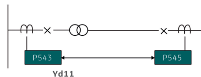
Figure 4 Application to transformer feeders
