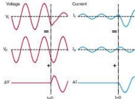
Relationship between superimposed and faulted power system
