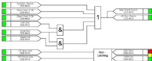
Programmable scheme logic
