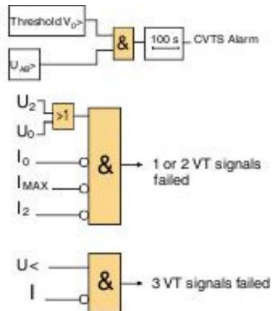
CVT & VT supervision
