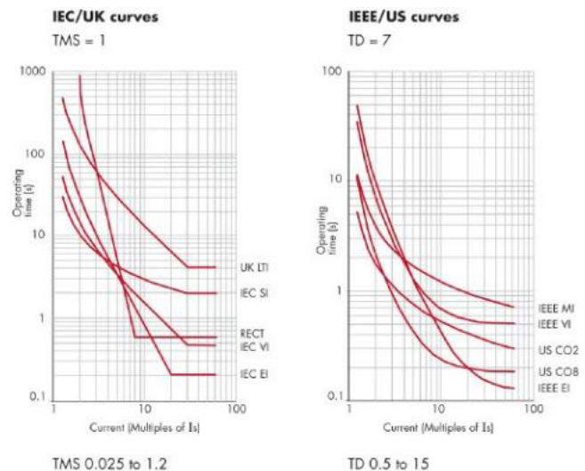
Choice of IDMT characteristics
