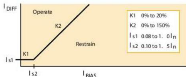
REF biased differential characteristics
