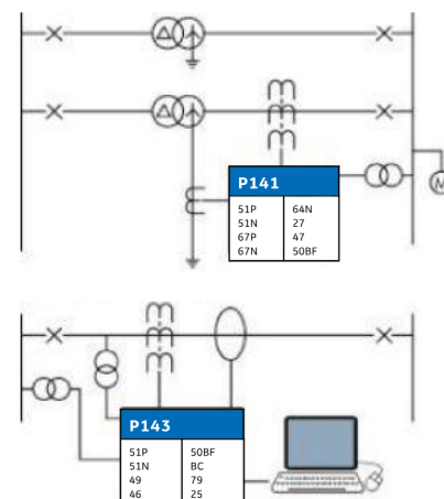
Typical applications of P14x
