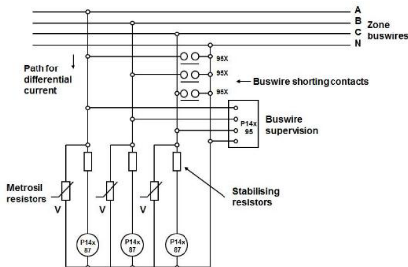
Typical high-impedance protection scheme - GE Vernova's P14x Agile relay provides full bus protection and scheme supervision
