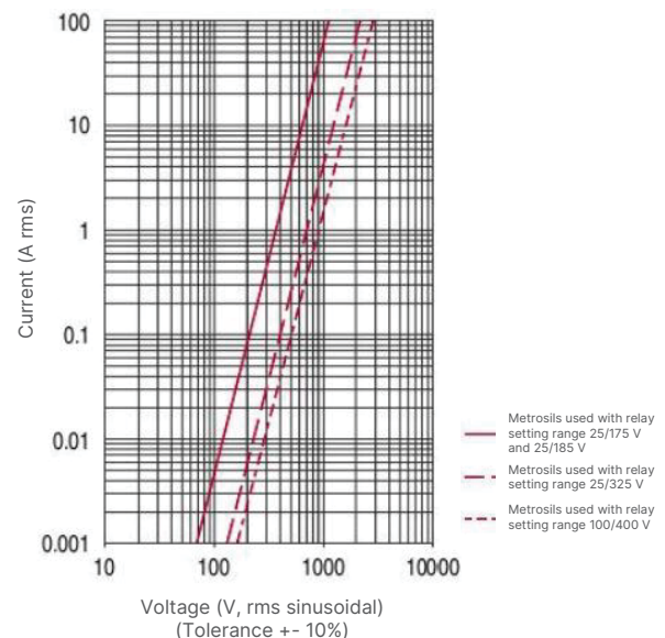
Figure 5 Nominal and extreme AC characteristics of external Metrosils for use with MFAC relays
