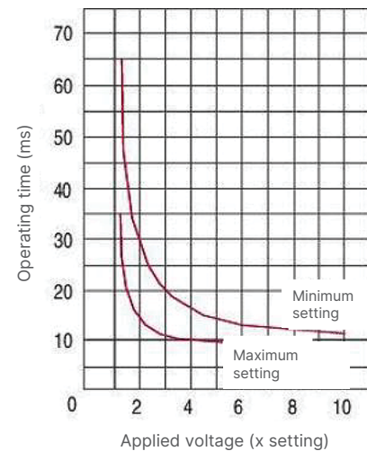
Figure 3: Typical time operating characteristics
