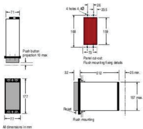
Figure 7 Case outline 15TE (size 3)
