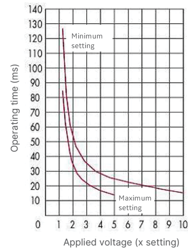
Figure 4 Typical time operating characteristics for 15-185 V relays only
