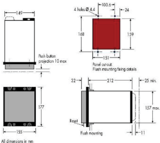
Figure 8 Case outline 30TE (size 6)
