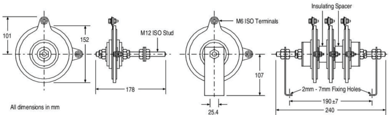
Figure 6 Outlines of external Metrosil units
