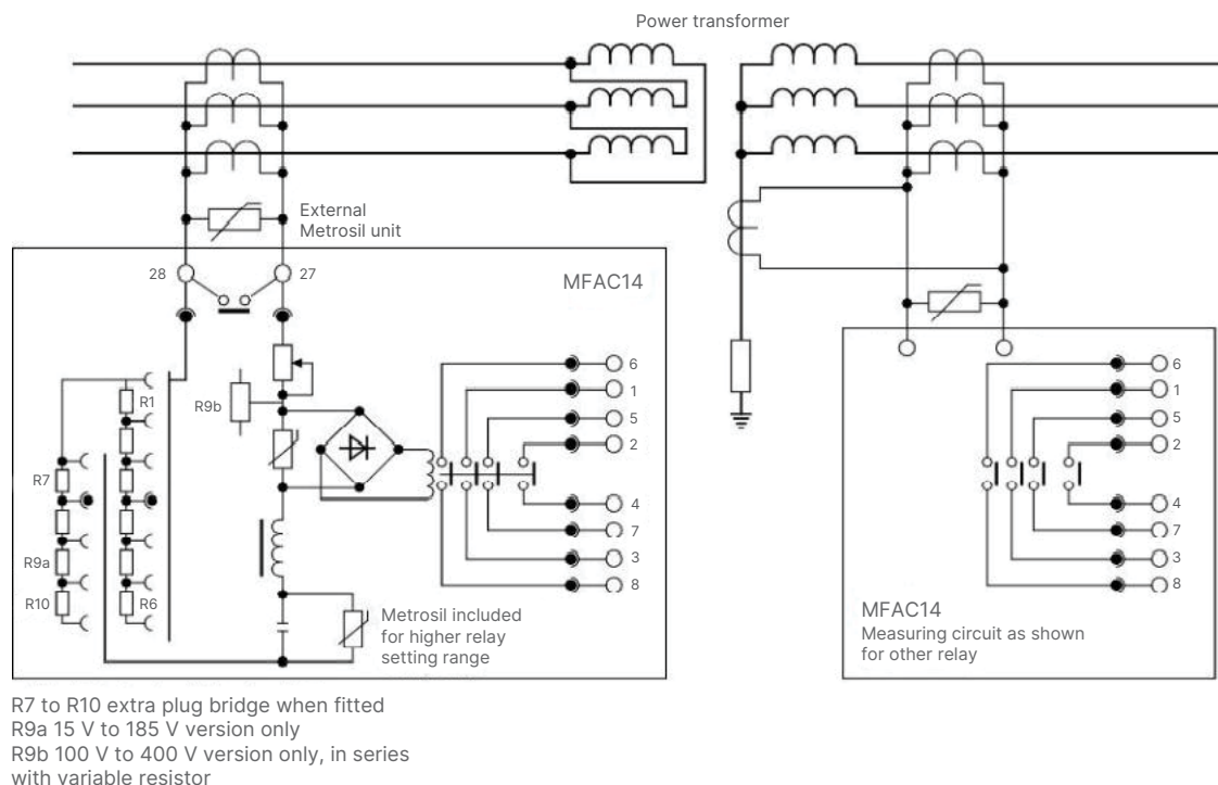
Figure 1 Type MFAC 14 relays applied to restricted earth fault protection of power transformer windings
