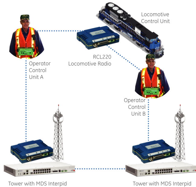
Figure 1: Freight Train/Rail Yard Application
