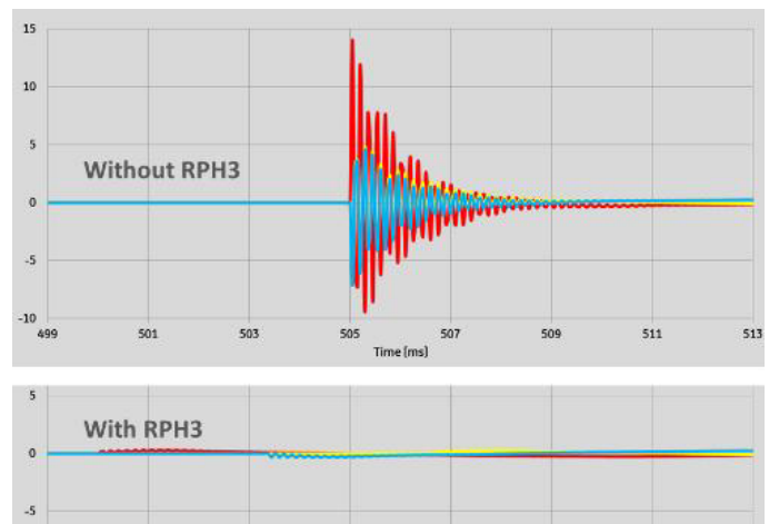
Inrush current limitation for shunt capacitor banks
