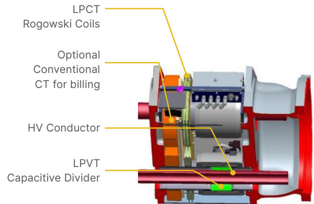
Combined Current and Voltage Transformer including an optional conventional core for billing function
