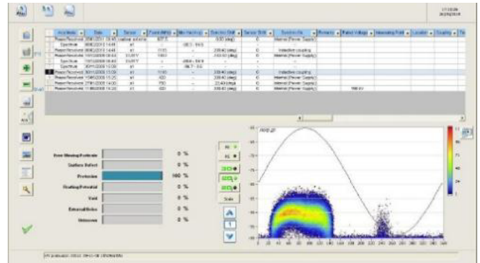
Time domain acquisition for pattern recognition with «PDWatch manager»
