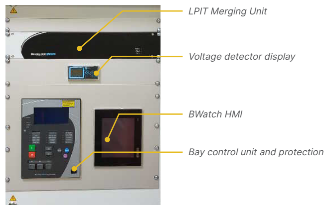
Digital Local Control Cubicle
