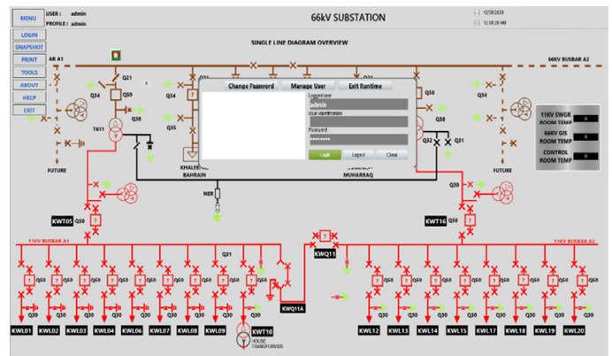
Figure 5: An SLD on a 66kV/11kV-substation project Pixel-based UI customization
