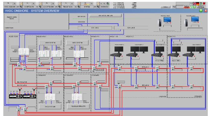
Figure 4: The IT system topology overview in a large offshore wind farm project
