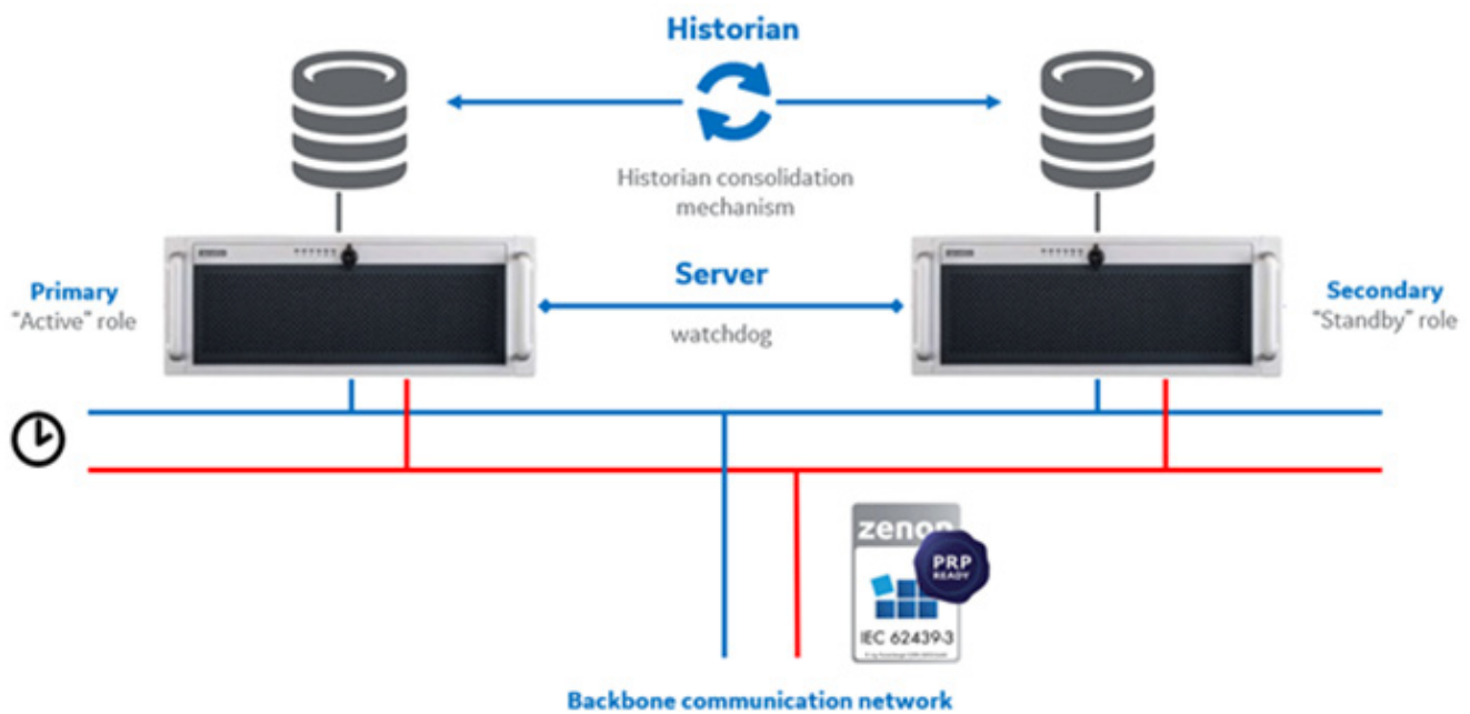
Figure 6: Server and data historian redundancy mechanisms, ensuring the high availability of data
