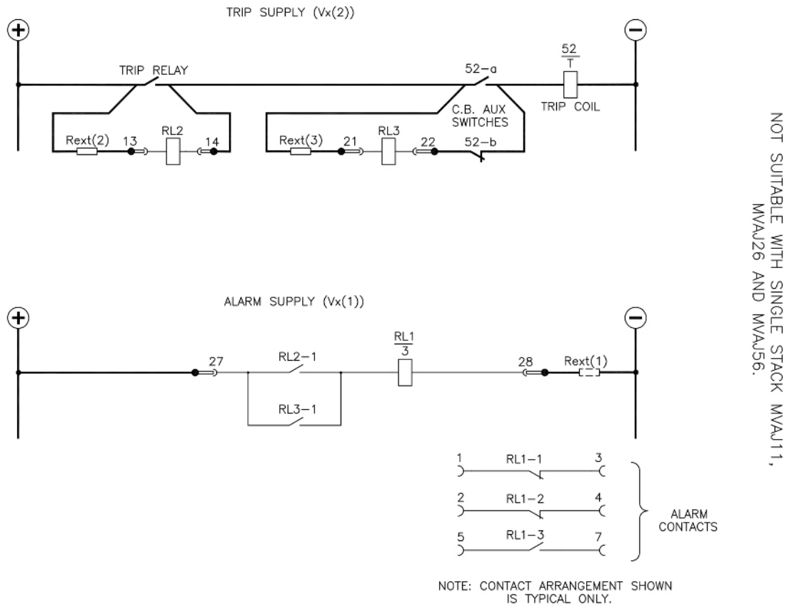
Figure 2 (c) MVAX 31 trip circuit supervision
