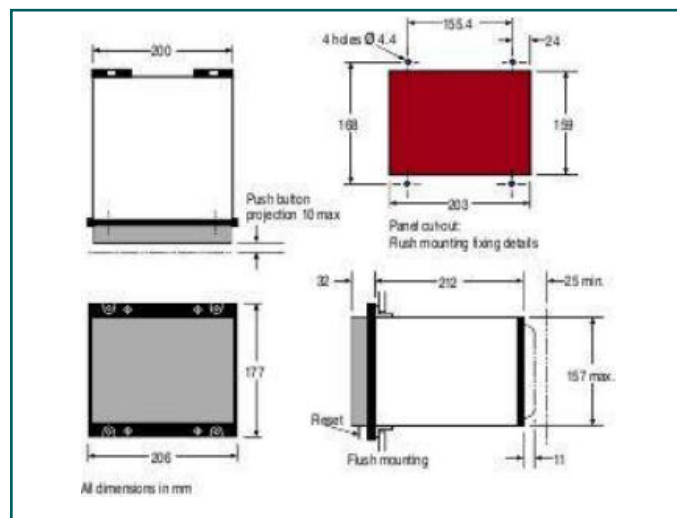
Figure 5 Case outline size 8
