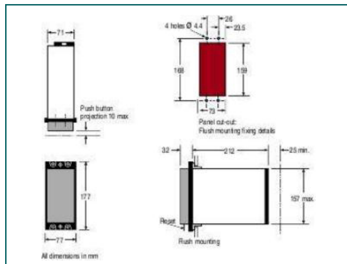
Figure 4 Case outline size 3
