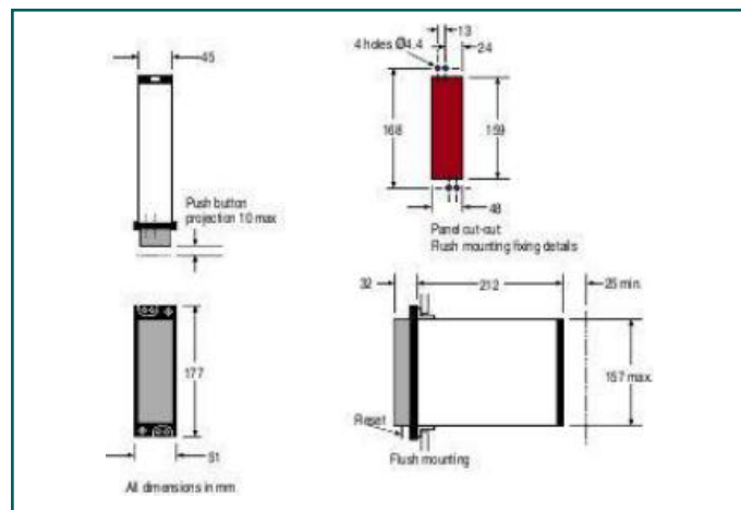
Figure 3 Case outline size 2
