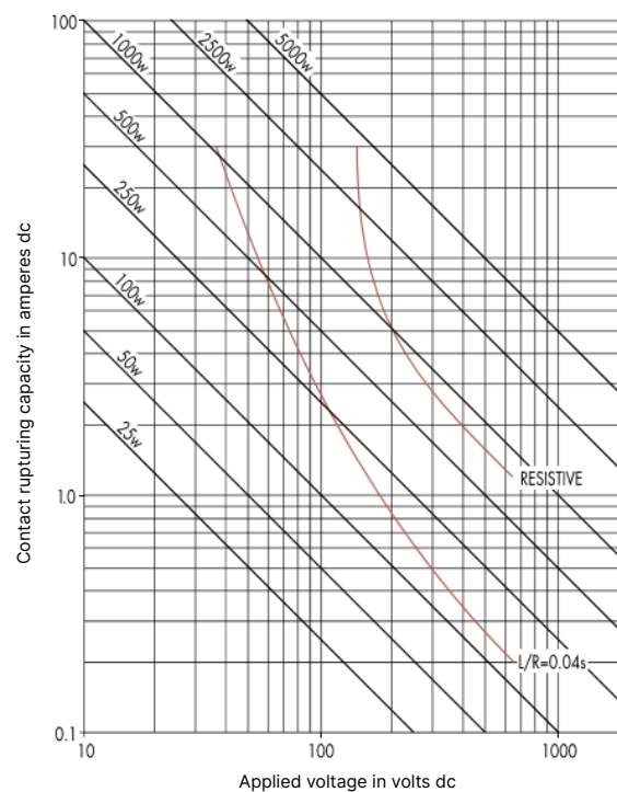
Figure 1 Breaking capacity curves of heavy duty blow-out contacts
