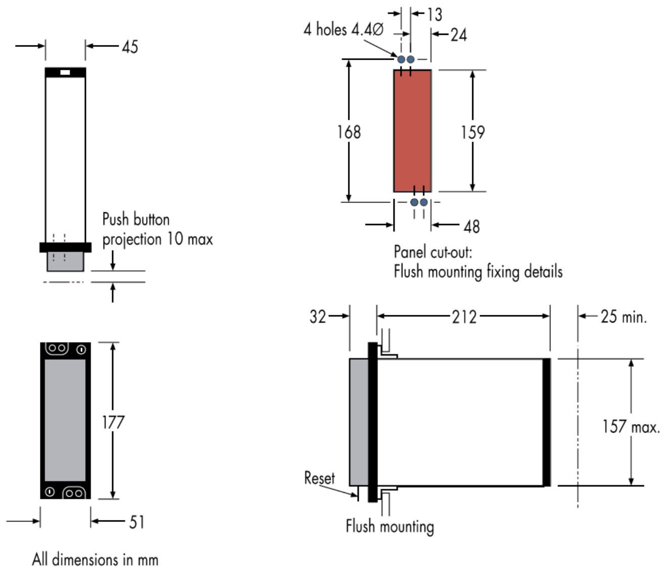
Figure 4: Case outline size 2
