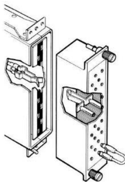
Figure 1 MMLG 01 test block and multi-finger test plug MMLB 01 (not inserted) with a CT shorting link
