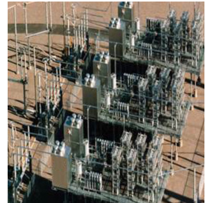
Series Compensation Bank
