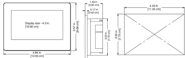
P70N - Color Touchscreen LCD Display
