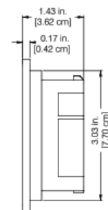
P70N Side Dimensions
