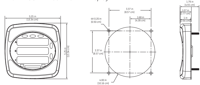
P40NPLUS - Three Line LED Display
