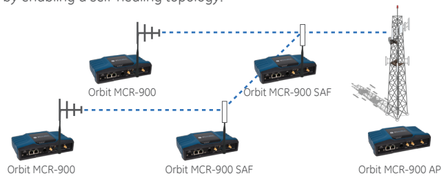
Figure 3: SAF physically extends the network range via a “daisy chain” topology
