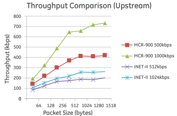
Figure 2: iNET II and Orbit MCR-900 Throughput Performance Comparison
