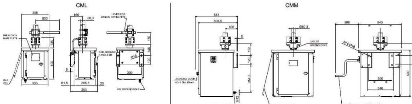
CML manual lever operating mechanism
