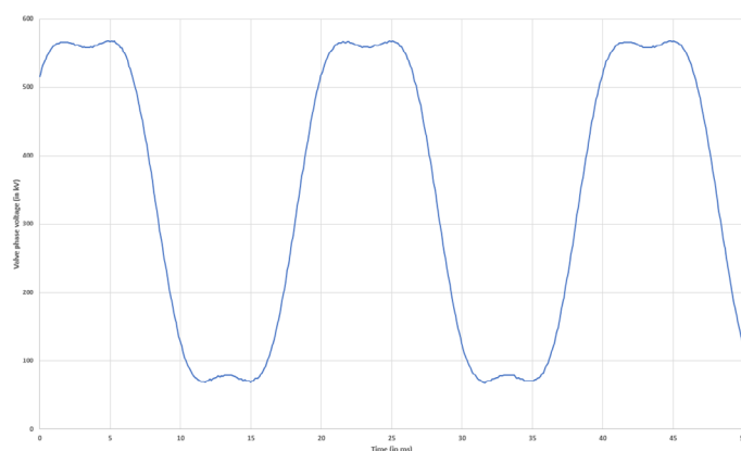
Measured valve phase voltage from DoWin 3 showing fundamental waveform with 3rd harmonic injection
