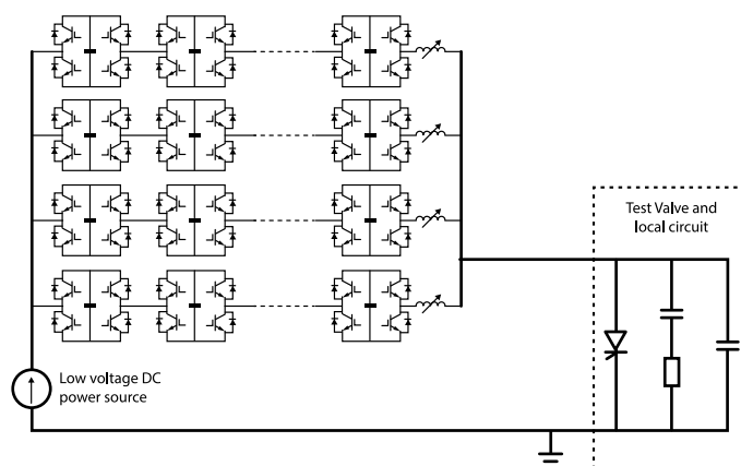
Simplified circuit diagram of the Valve Test Facility
