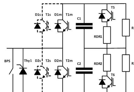
Simplified Circuit Diagram of Valve Submodule
