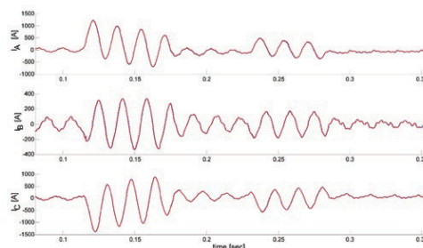
Figure 5. On Sept. 30, 2008 event – Hyatt line currents: hardwired relay (blue) and measured by HardFiber bricks (red). The resulting pink color is due to exact overlay of traces.
