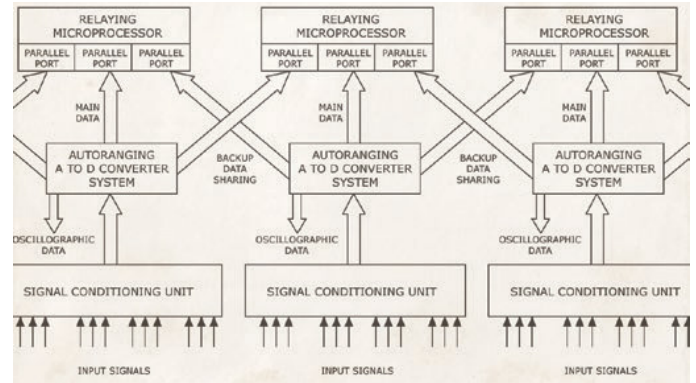
Figure 3. AEP digital substation architecture concept, circa 1980.
