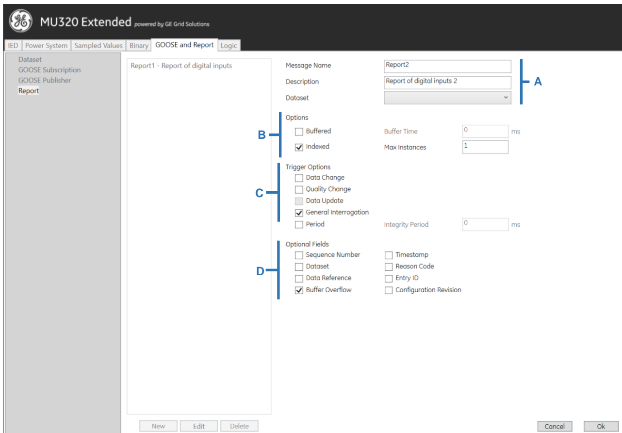
GOOSE Publisher Configuration Screen
