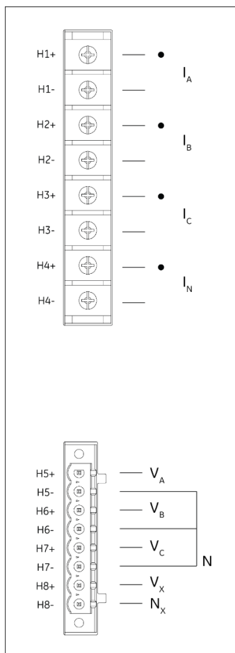
Voltage and current analog inputs
