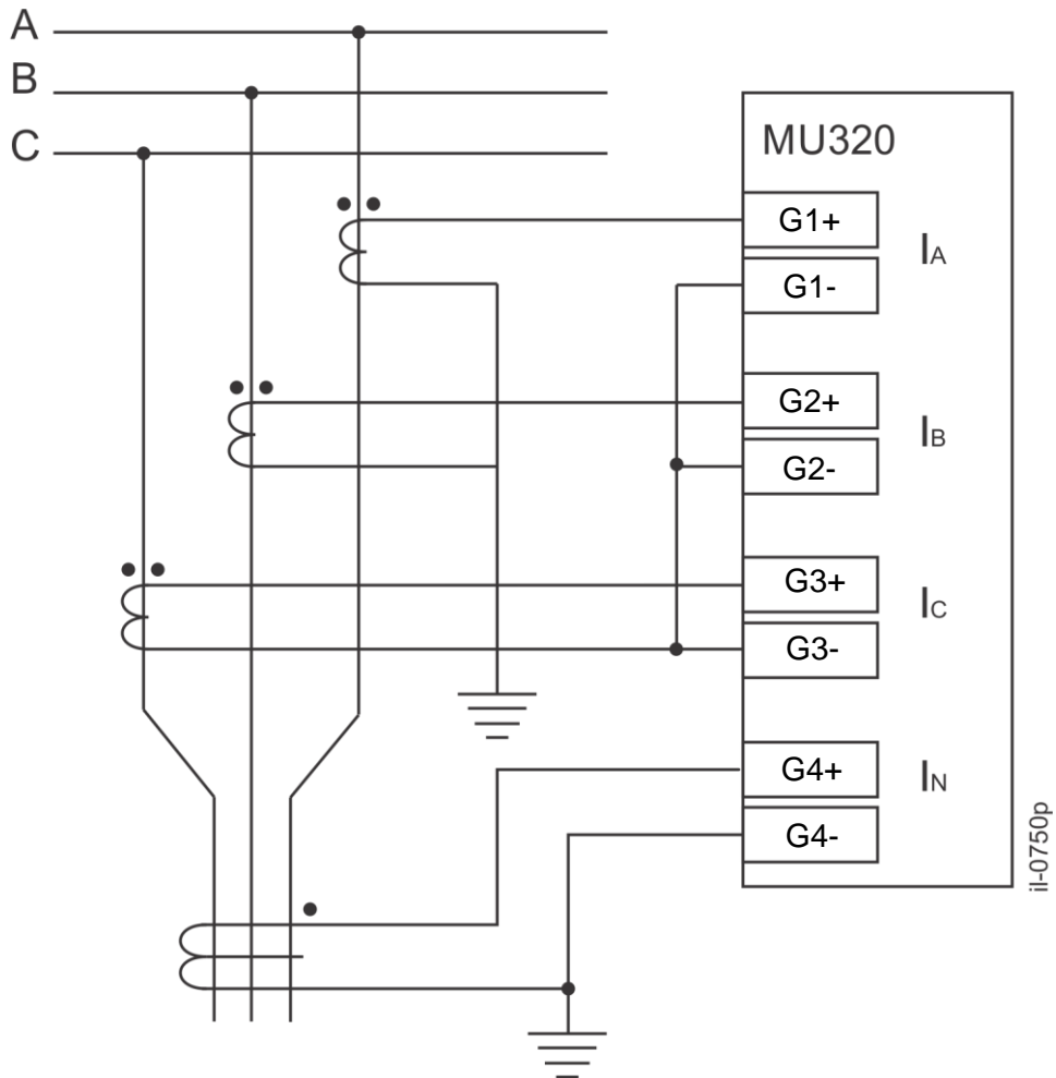
Typical current connection diagram with I_N from the residual CT
