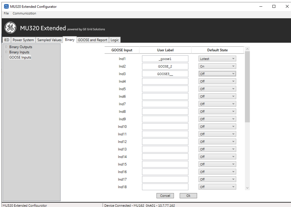
GOOSE Inputs Configuration
