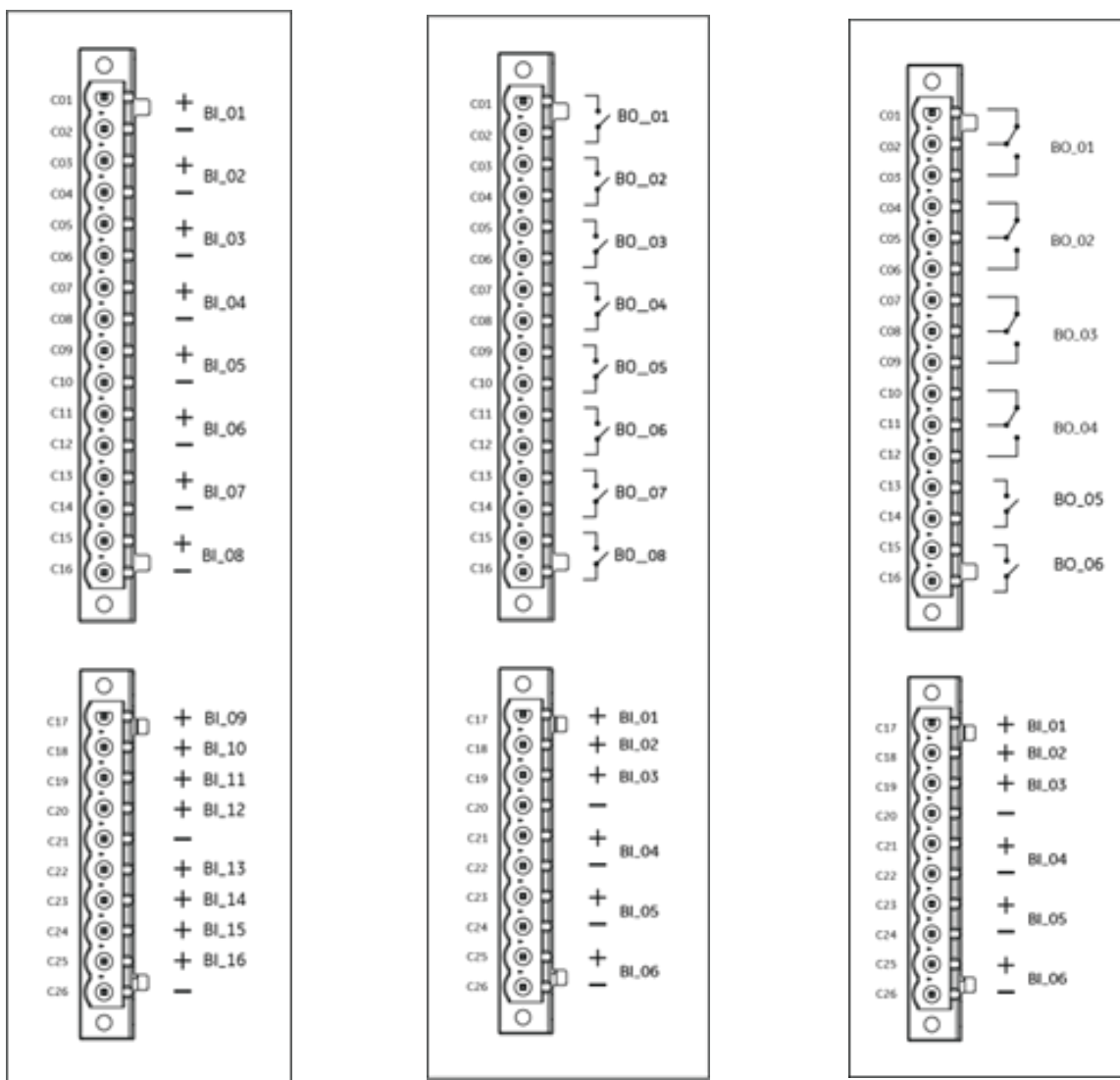
Binary board model B3
