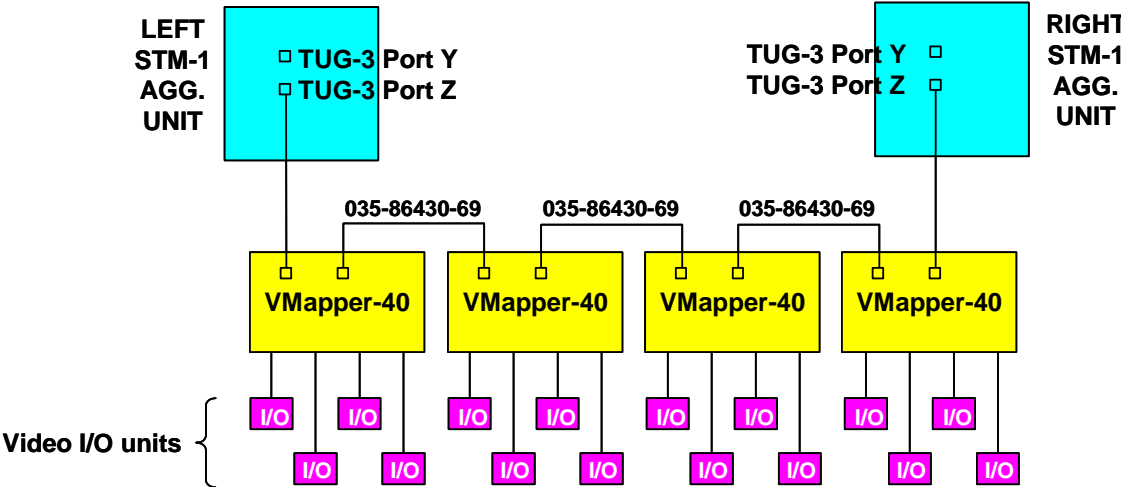
Figure 4: Cascading VMapper-40 Units
