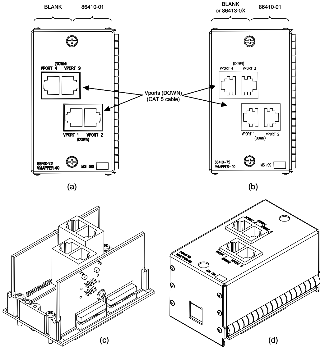
Figure 6: VMapper-40 Paddleboard Assemblies: (a) 86410-72; (b) 86410-75; (c) 3-D View without EMC Cover; (d) 3-D View with EMC Cover (86410-72)
