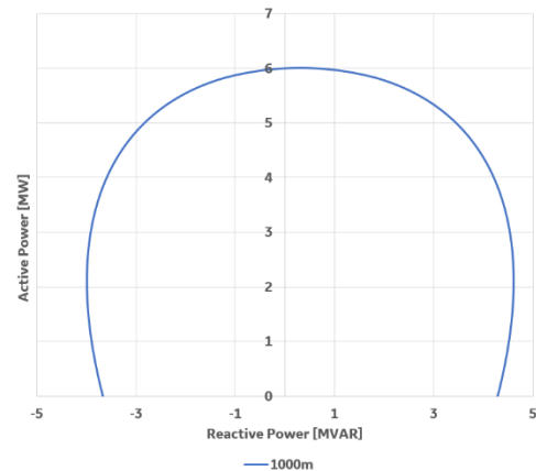
13. Sample PQ diagram for FLEXINVERTER 2090 at nominal grid voltage, 1400 Vdc and 35°C ambient
